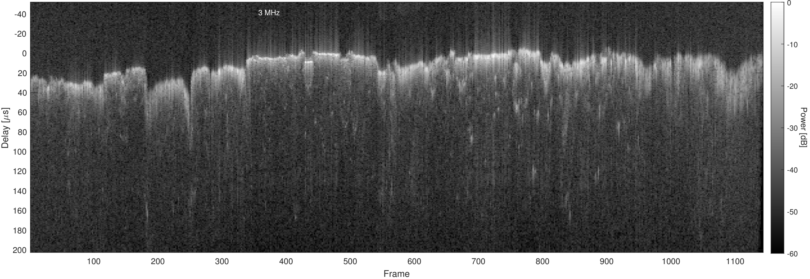
Orbit 11209, Chapman, No Window, Channel 2
