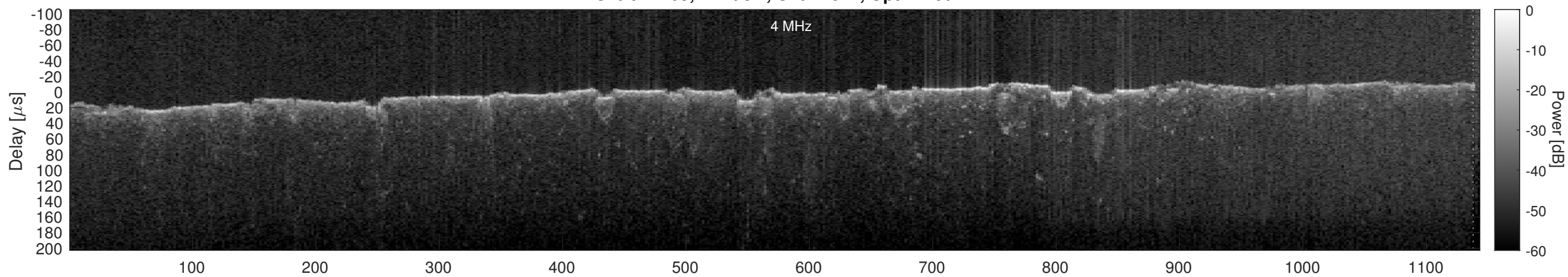
Orbit 11209, Cluttergram
