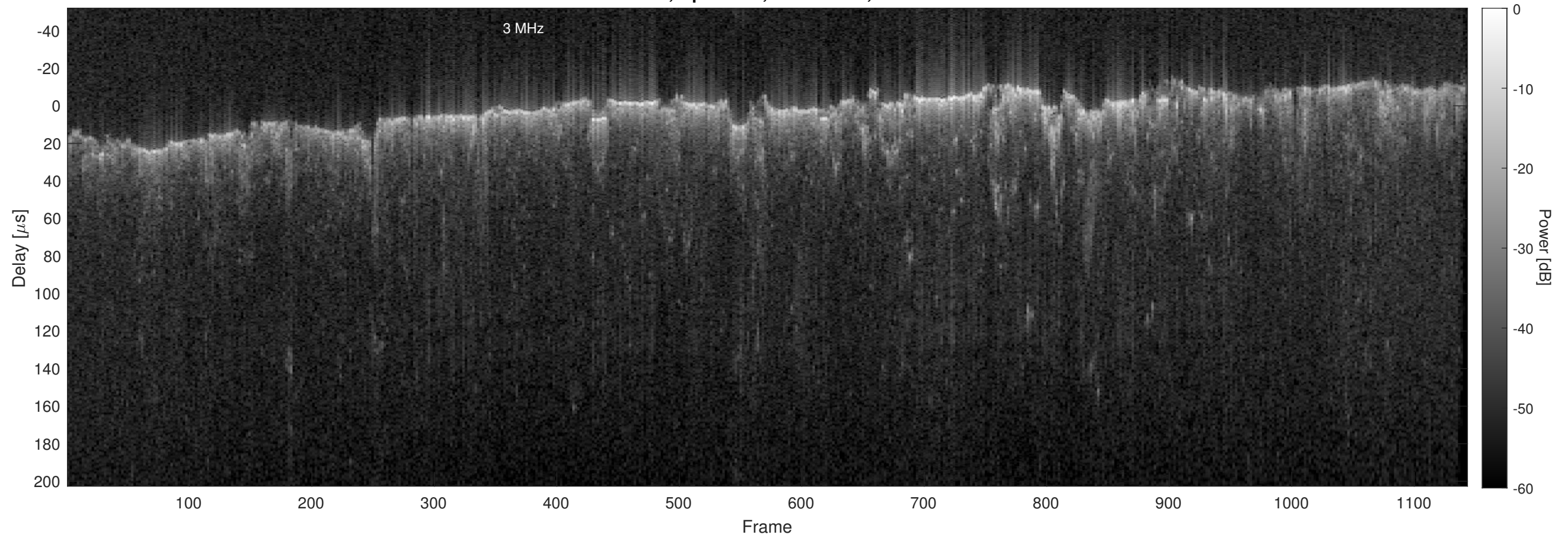
Orbit 11209, Optimized, No Window, Channel 2
