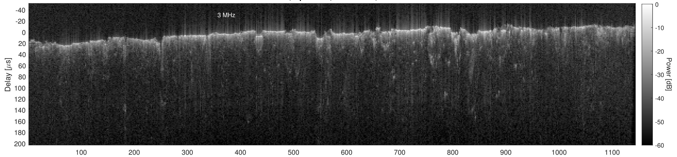
Orbit 11209, Cluttergram
