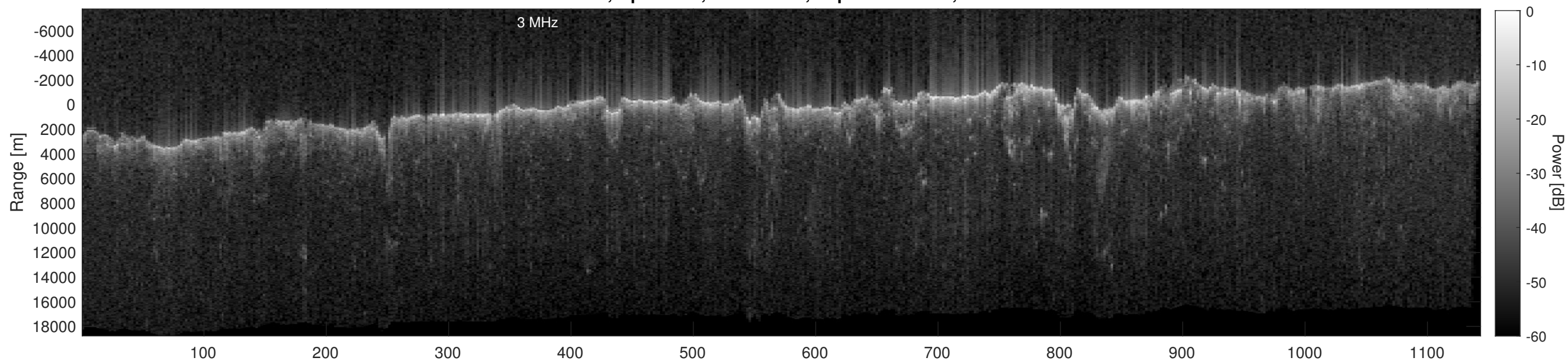
Orbit 11209, Depth-Corrected Cluttergram
