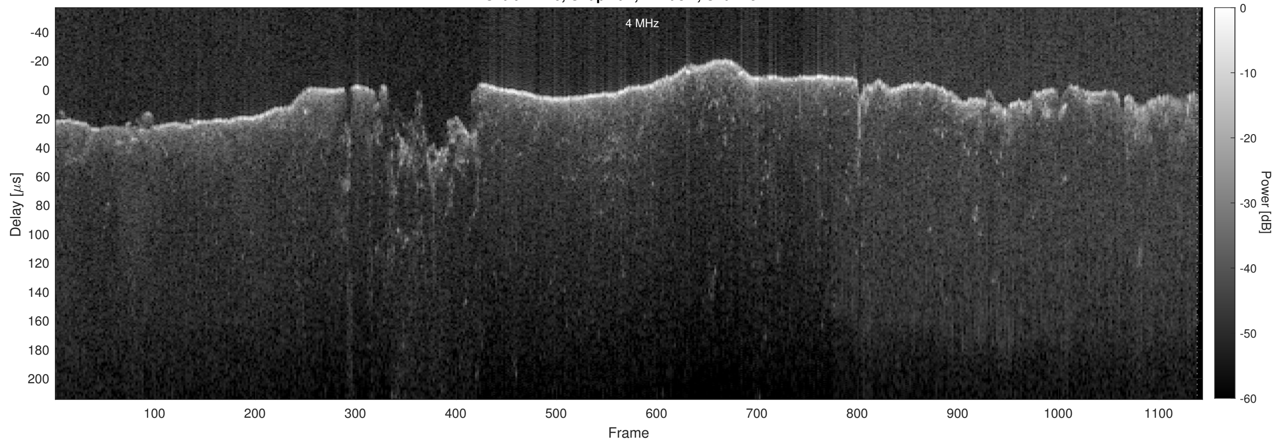
Orbit 11210, Chapman, Window, Channel 2
