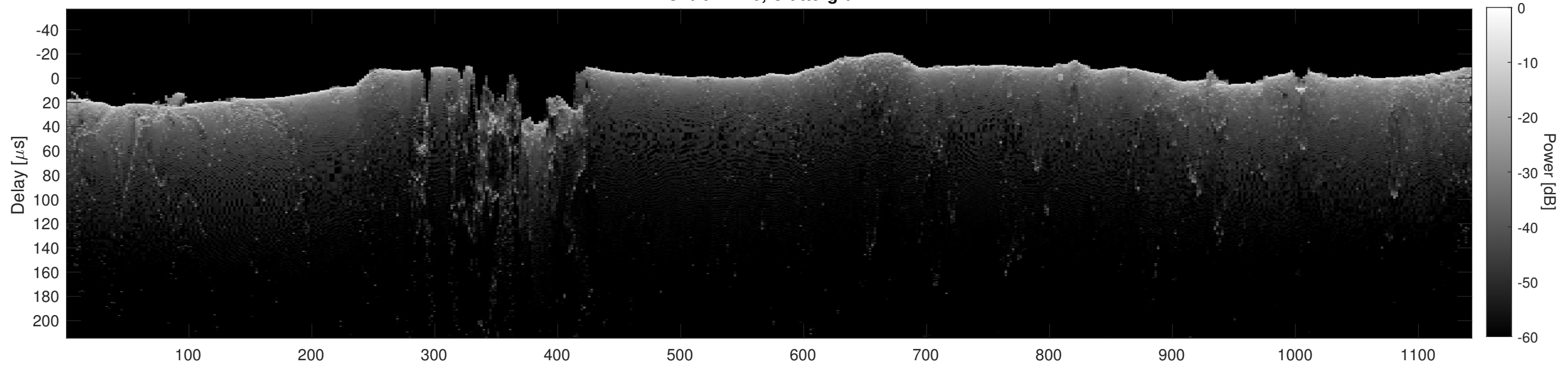
Orbit 11210, Cluttergram
