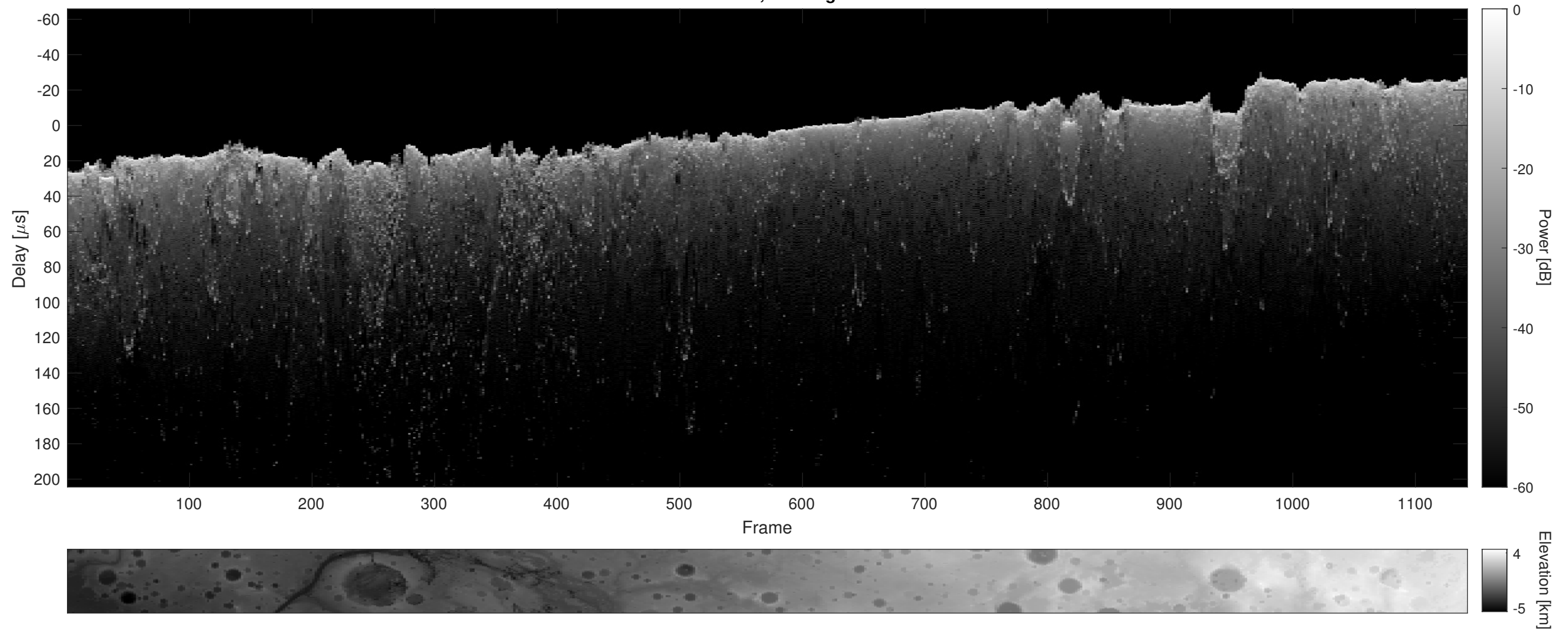
Orbit 11213, Cluttergram
