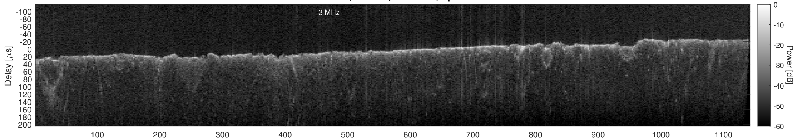
Orbit 11213, Cluttergram
