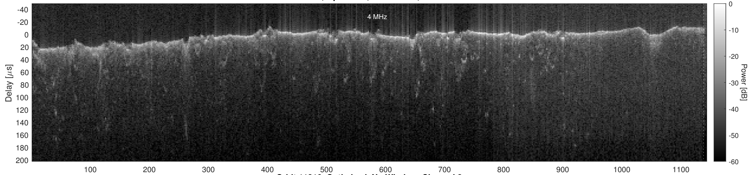
Orbit 11216, Optimized, No Window, Channel 2
