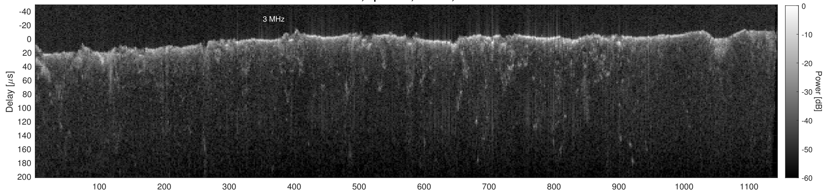
Orbit 11216, Cluttergram
