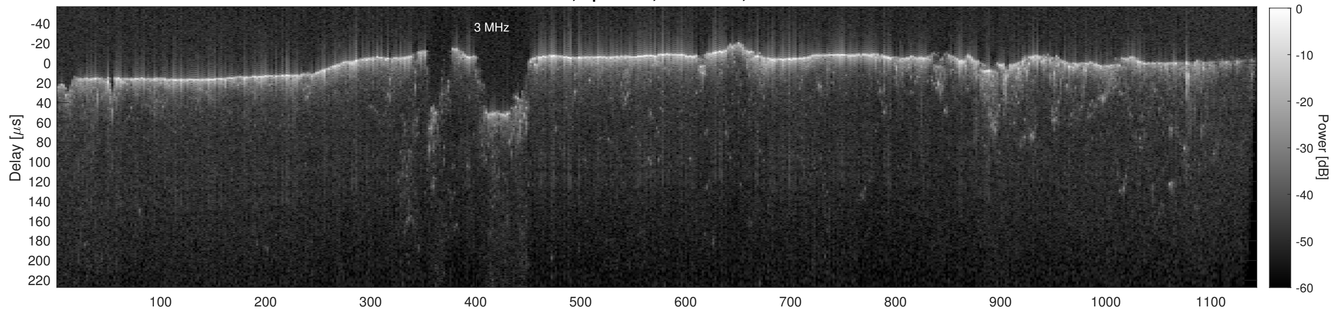
Orbit 11217, Cluttergram
