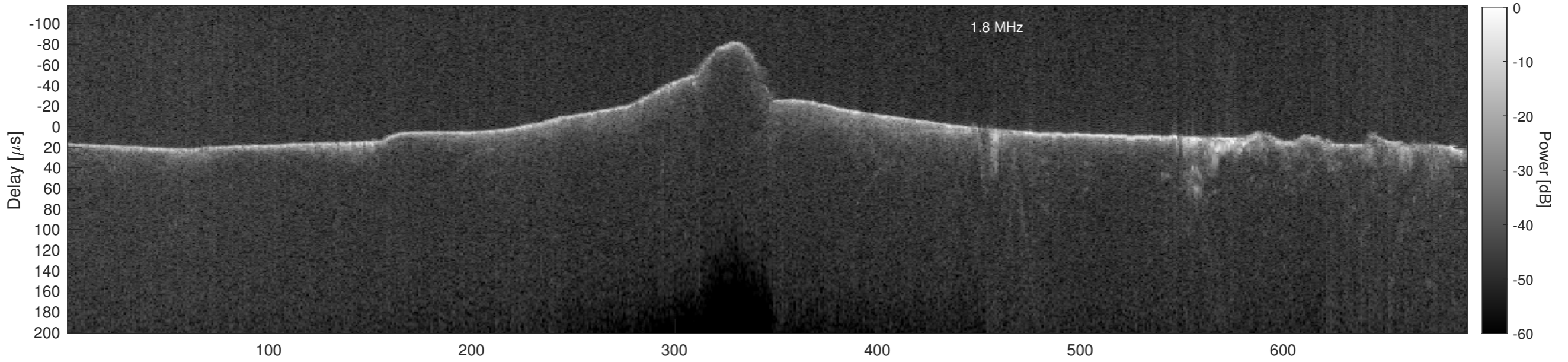
Orbit 11221, Cluttergram
