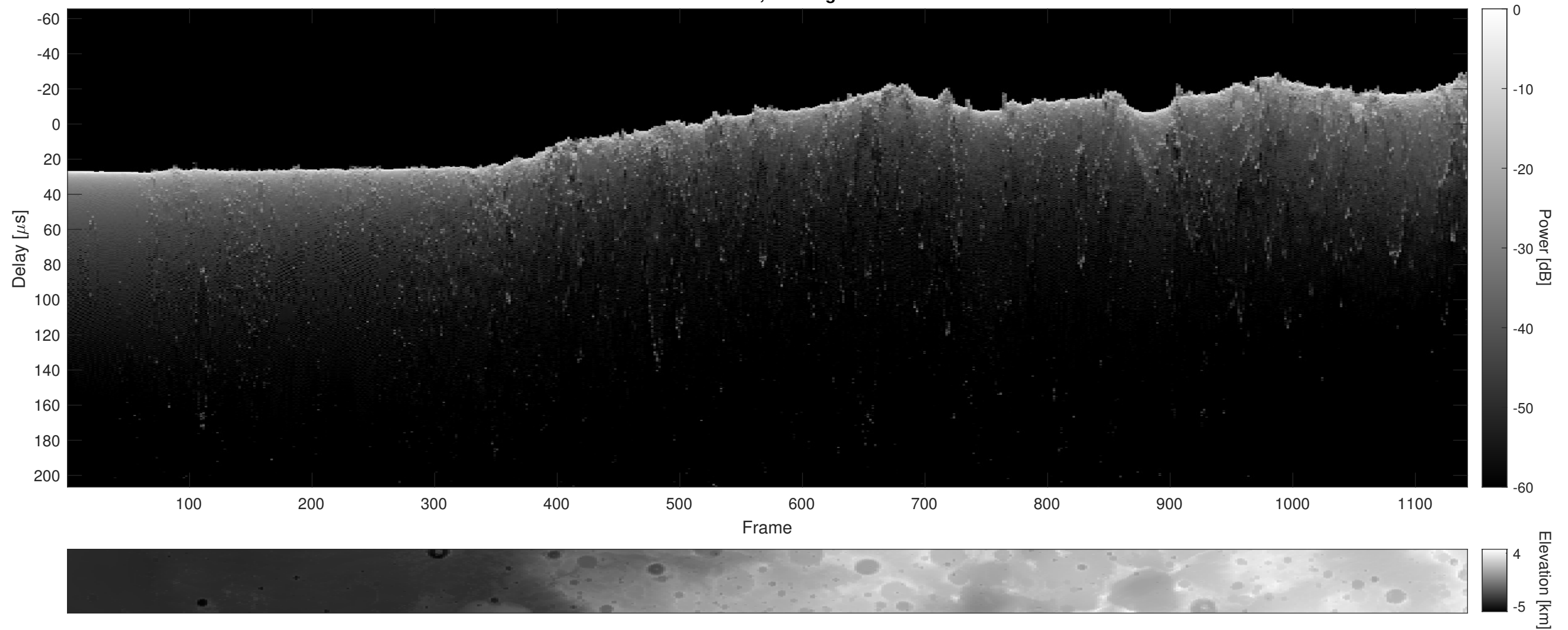
Orbit 11225, Cluttergram
