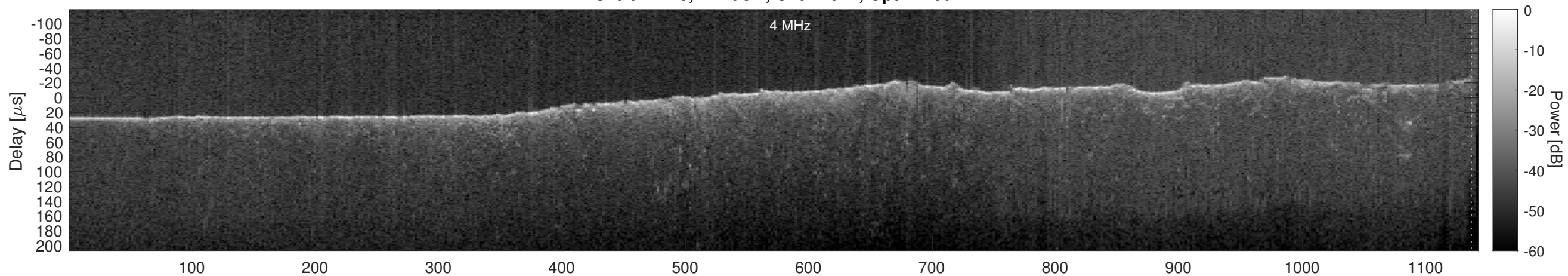
Orbit 11225, Cluttergram
