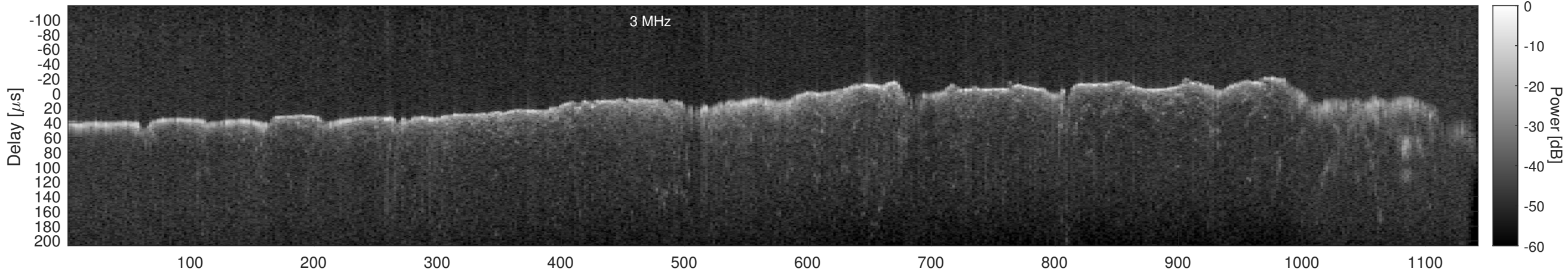
Orbit 11225, Window, Channel 2, Chapman
