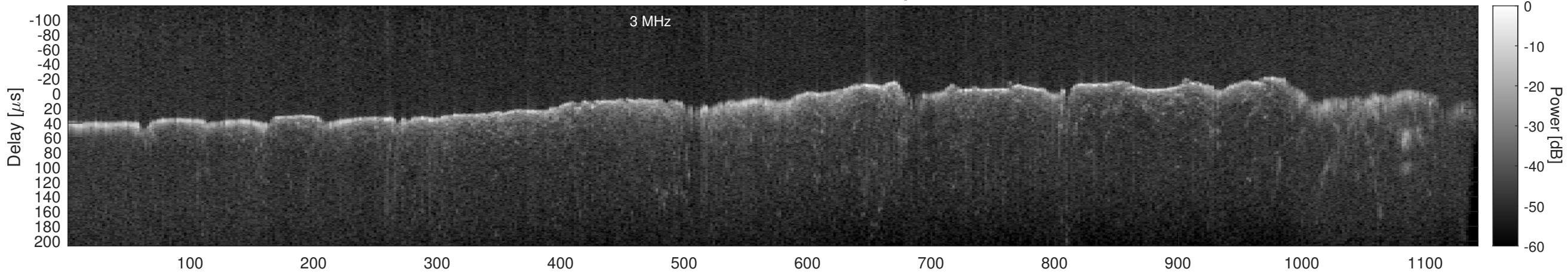
Orbit 11225, Window, Channel 2, Optimized
