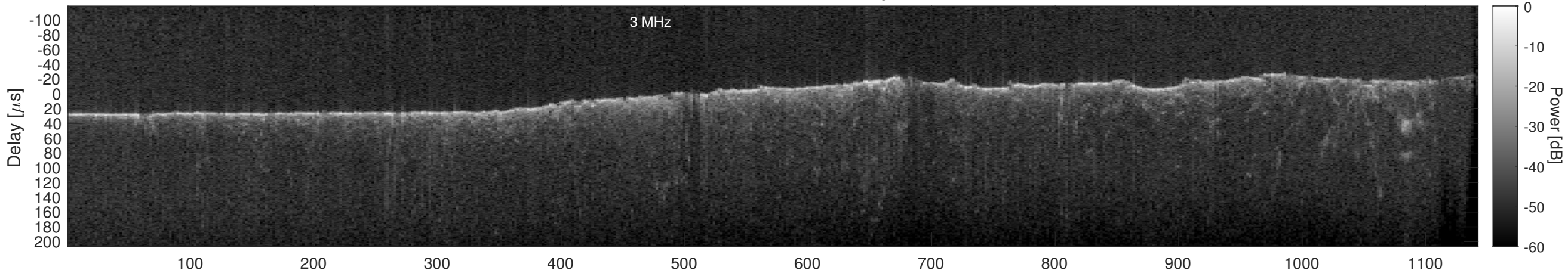
Orbit 11225, Cluttergram
