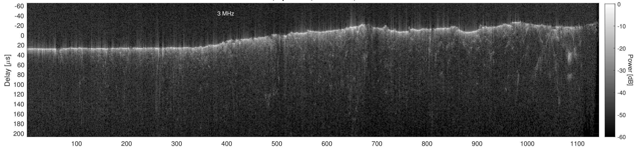
Orbit 11225, Cluttergram
