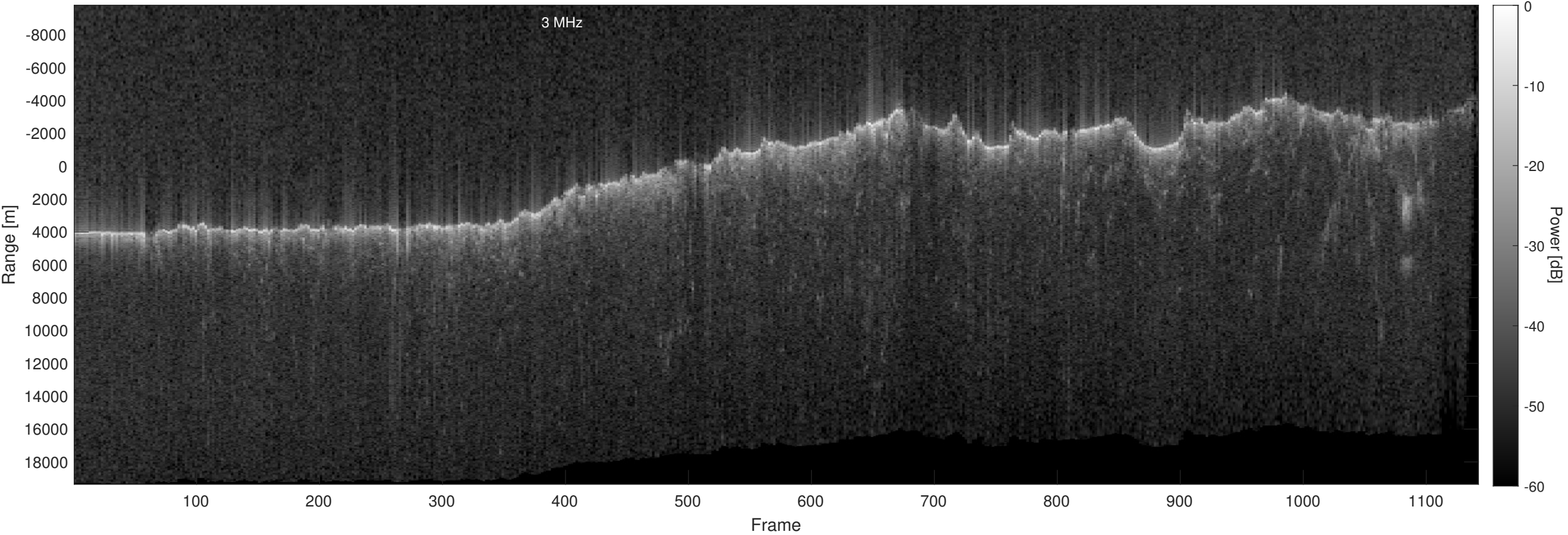
Orbit 11225, Optimized, No Window, Depth-Corrected, Channel 2
