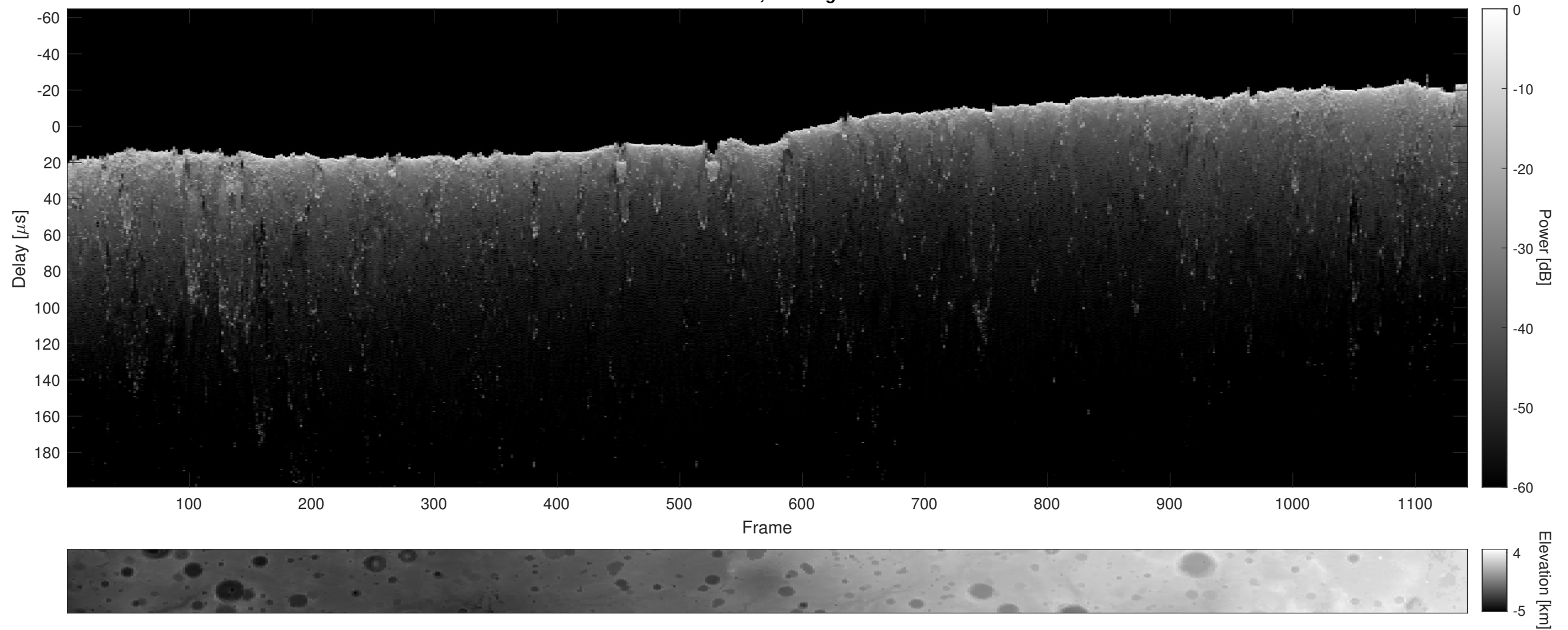
Orbit 11227, Cluttergram
