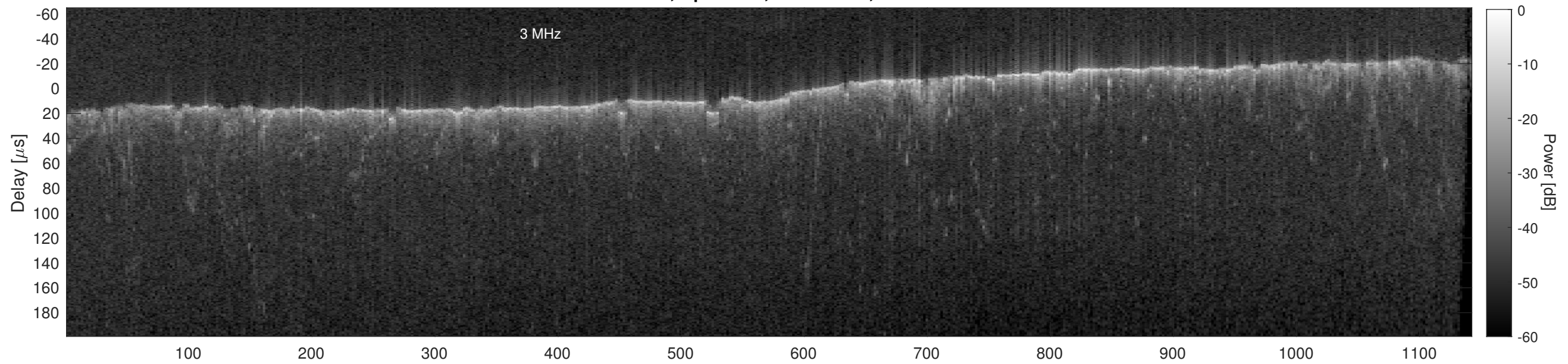
Orbit 11227, Cluttergram
