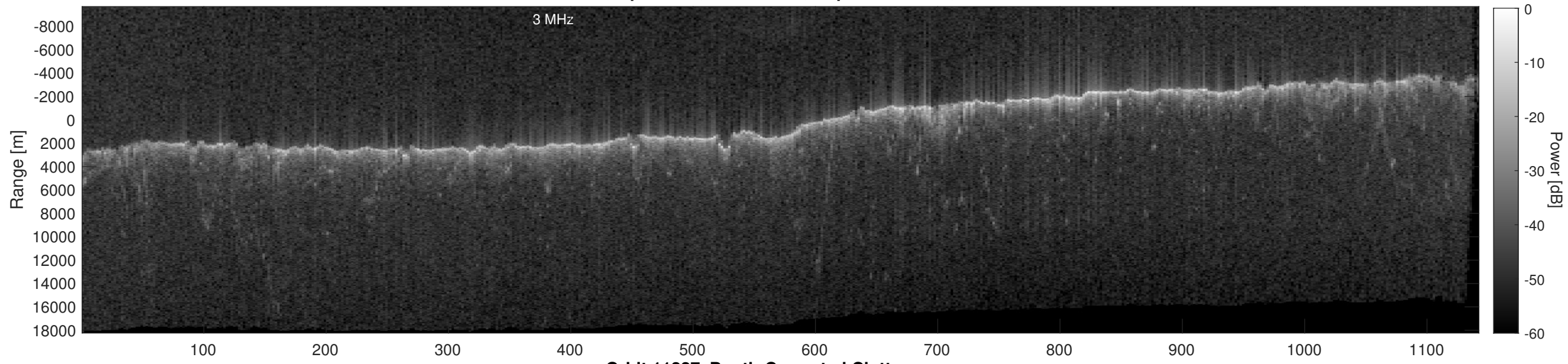
Orbit 11227, Depth-Corrected Cluttergram
