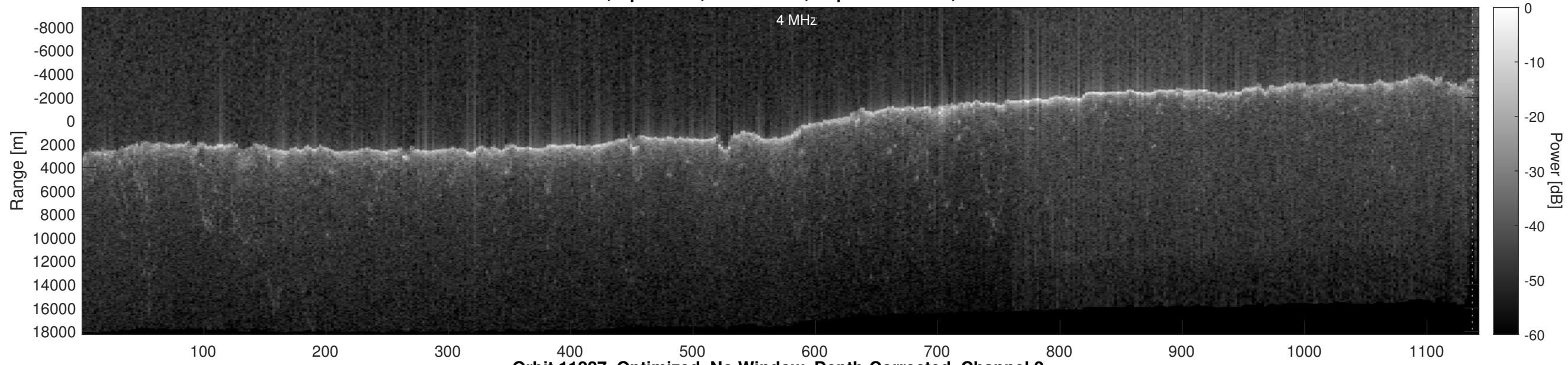
Orbit 11227, Optimized, No Window, Depth-Corrected, Channel 2
