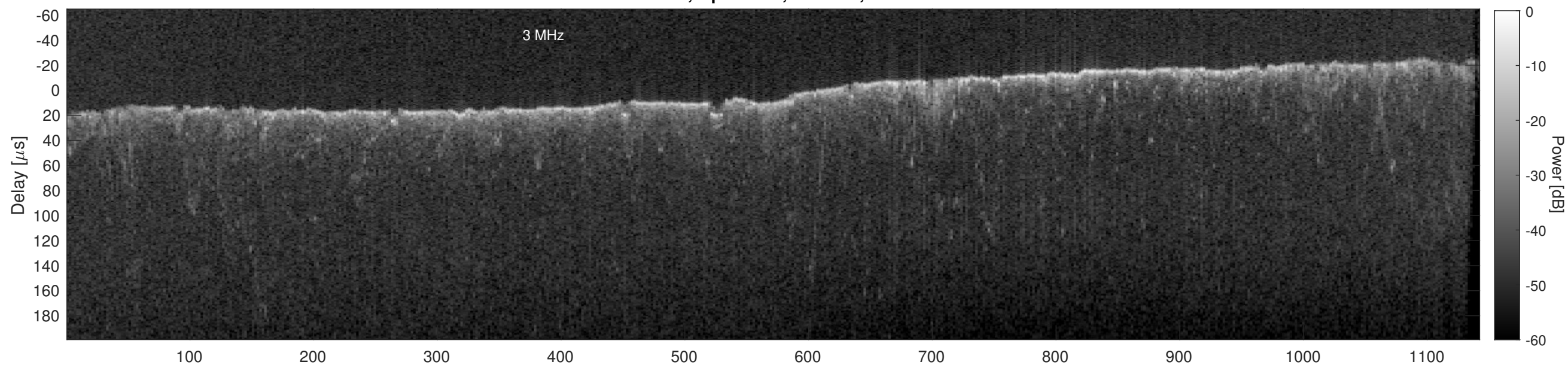
Orbit 11227, Cluttergram
