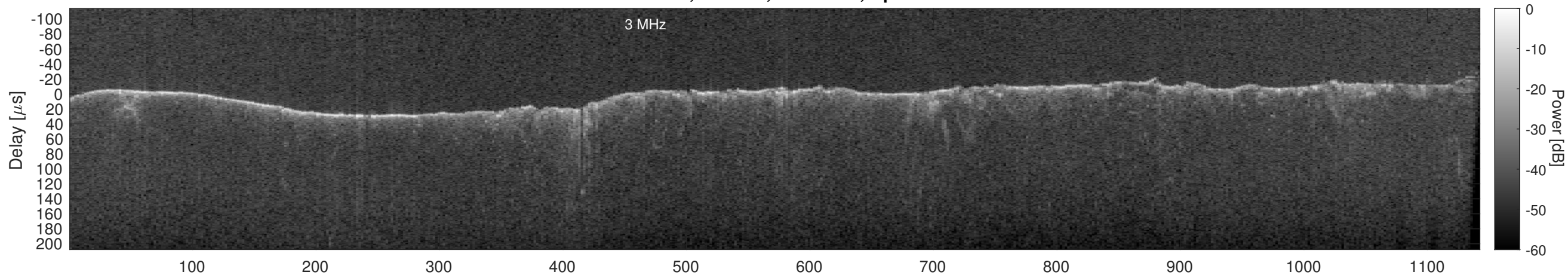
Orbit 11229, Cluttergram
