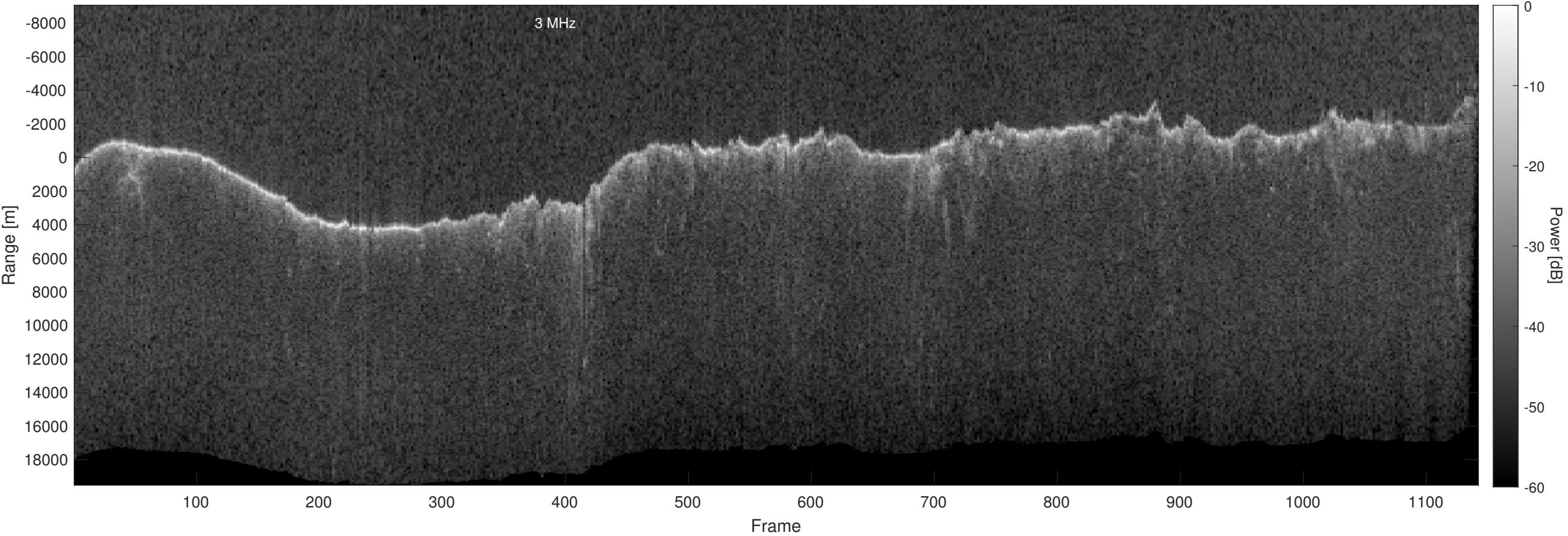
Orbit 11229, Optimized, Window, Depth-Corrected, Channel 2
