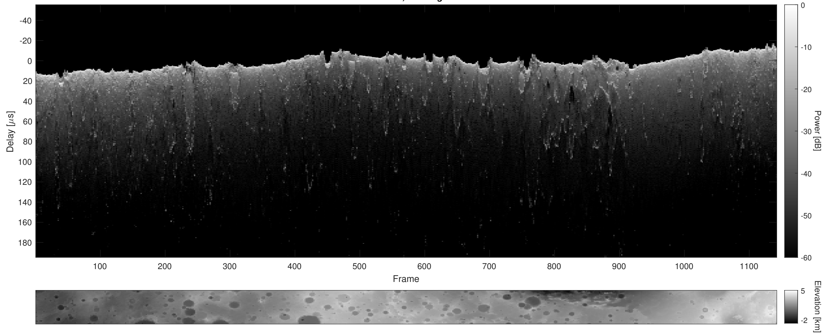
Orbit 11230, Cluttergram
