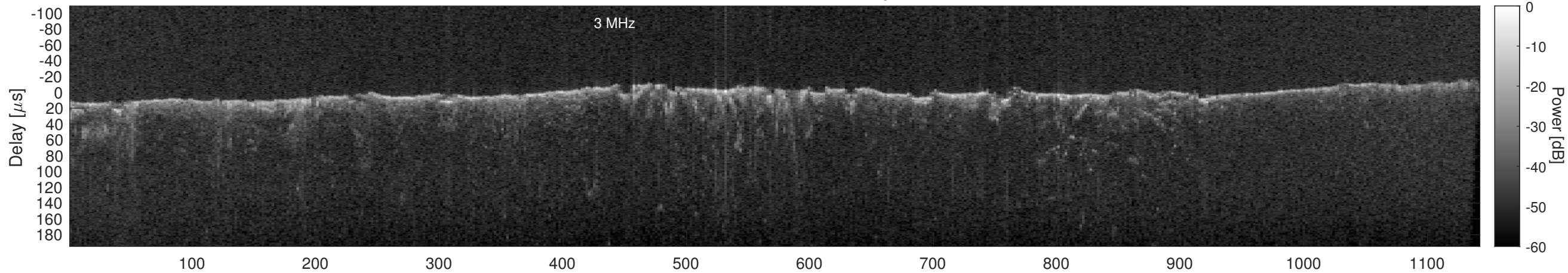
Orbit 11230, Cluttergram
