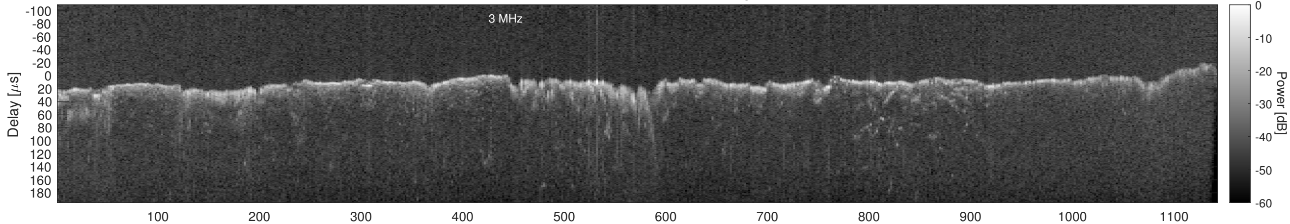
Orbit 11230, Window, Channel 2, Optimized
