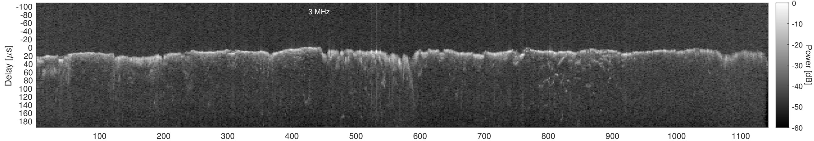
Orbit 11230, Window, Channel 2, Chapman
