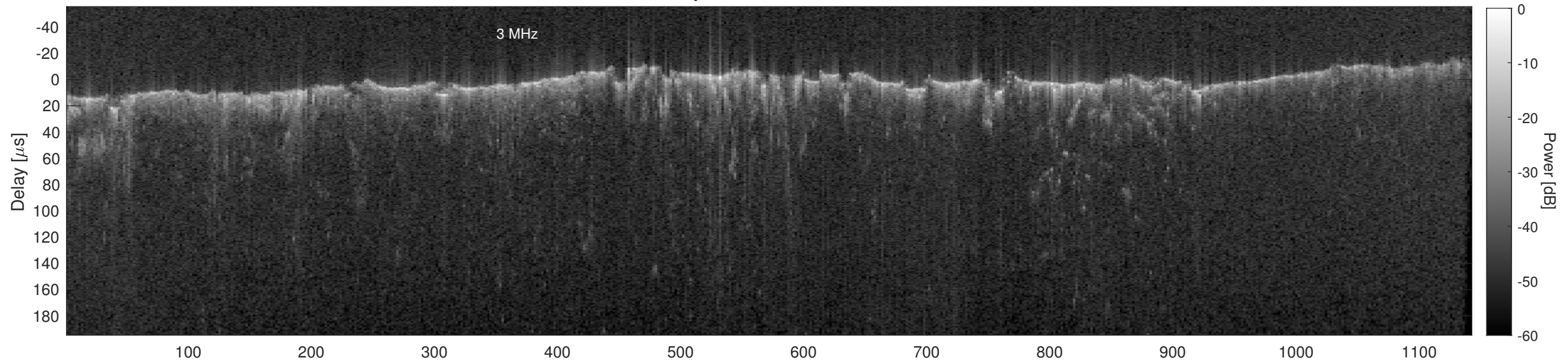
Orbit 11230, Cluttergram
