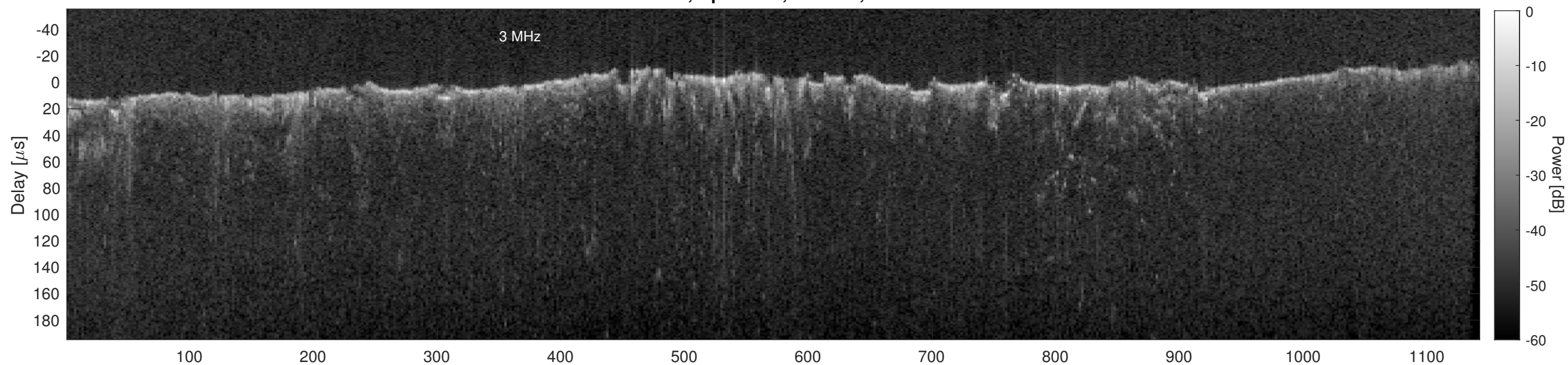
Orbit 11230, Cluttergram
