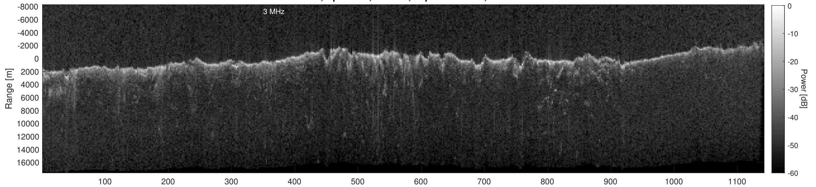
Orbit 11230, Depth-Corrected Cluttergram
