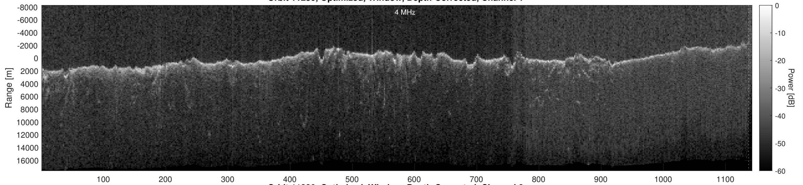
Orbit 11230, Optimized, Window, Depth-Corrected, Channel 2
