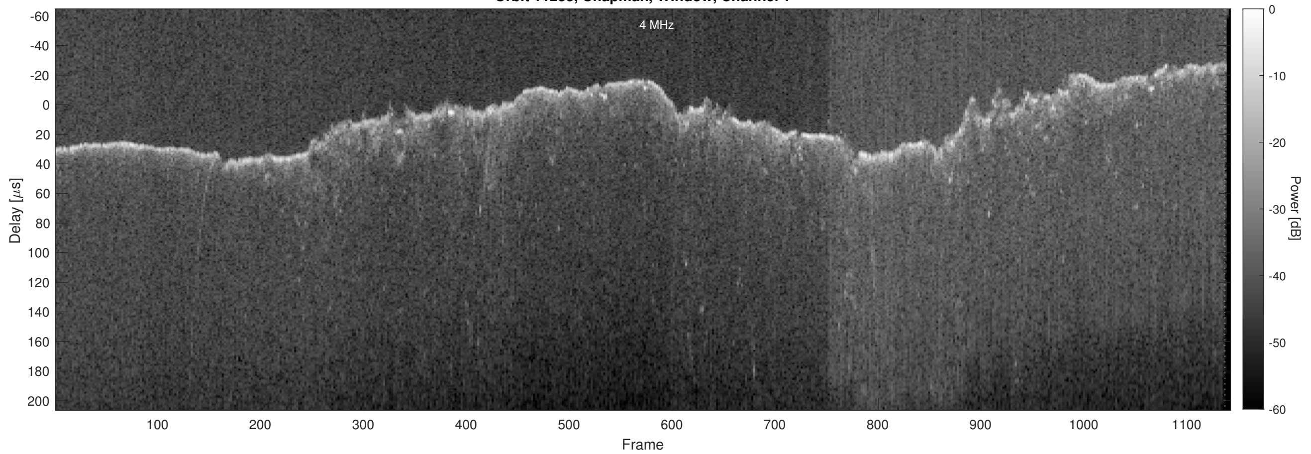
Orbit 11233, Chapman, Window, Channel 2
