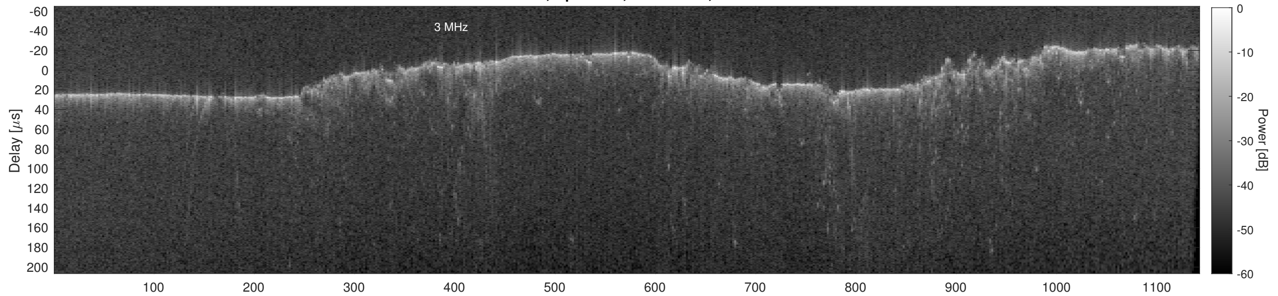
Orbit 11233, Cluttergram
