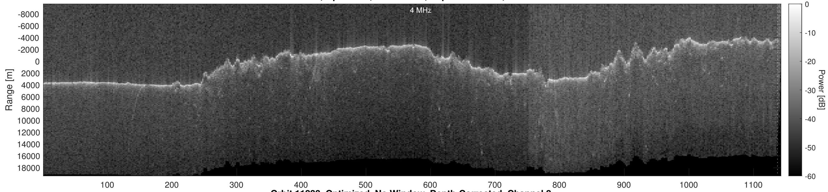
Orbit 11233, Optimized, No Window, Depth-Corrected, Channel 2
