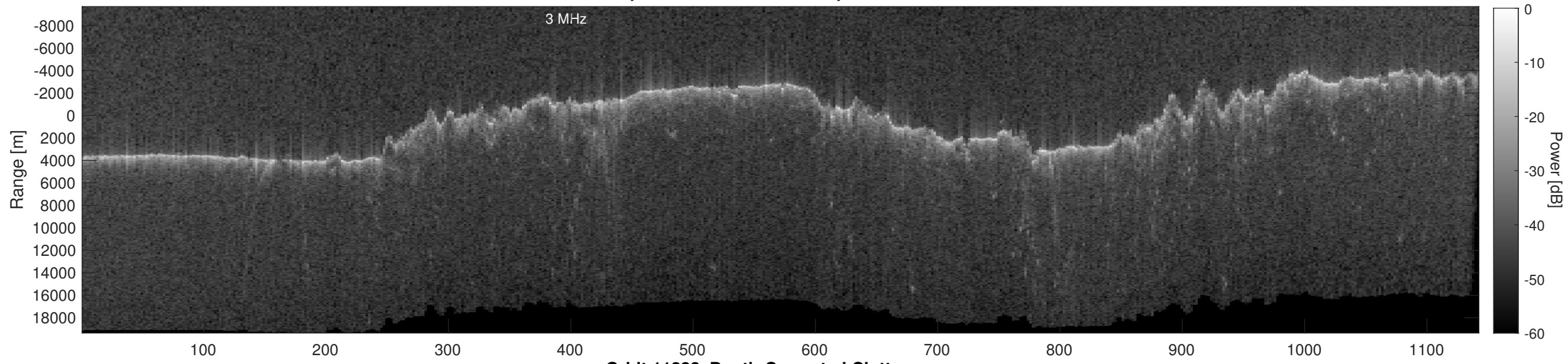
Orbit 11233, Depth-Corrected Cluttergram
