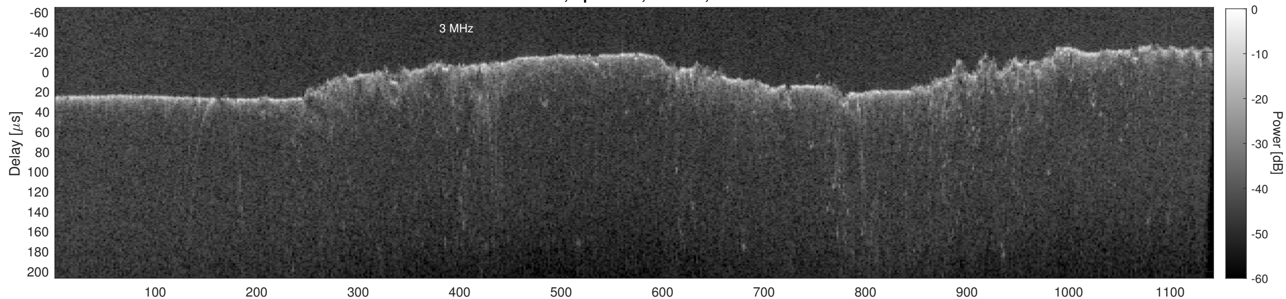
Orbit 11233, Cluttergram
