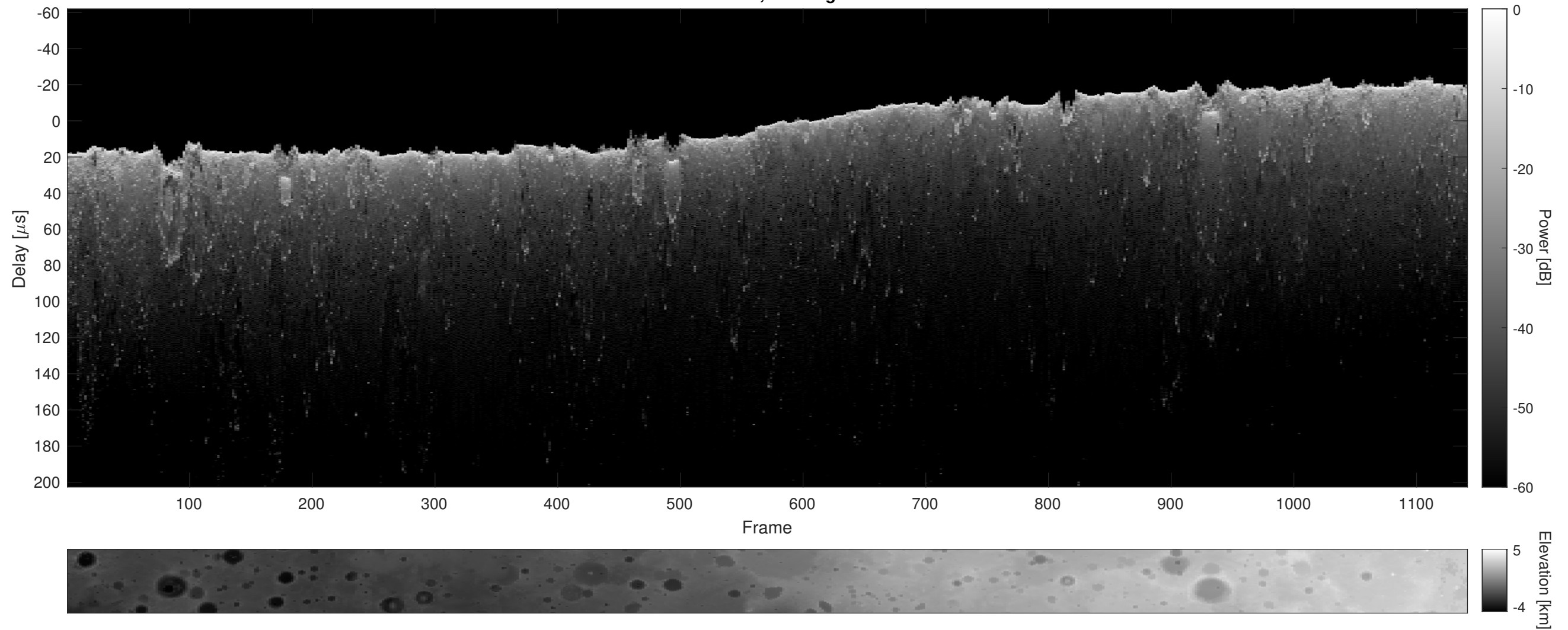
Orbit 11234, Cluttergram
