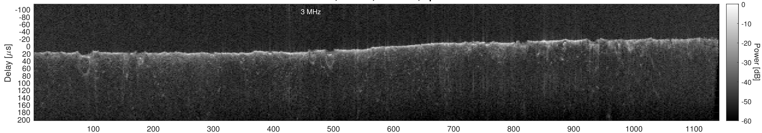
Orbit 11234, Cluttergram
