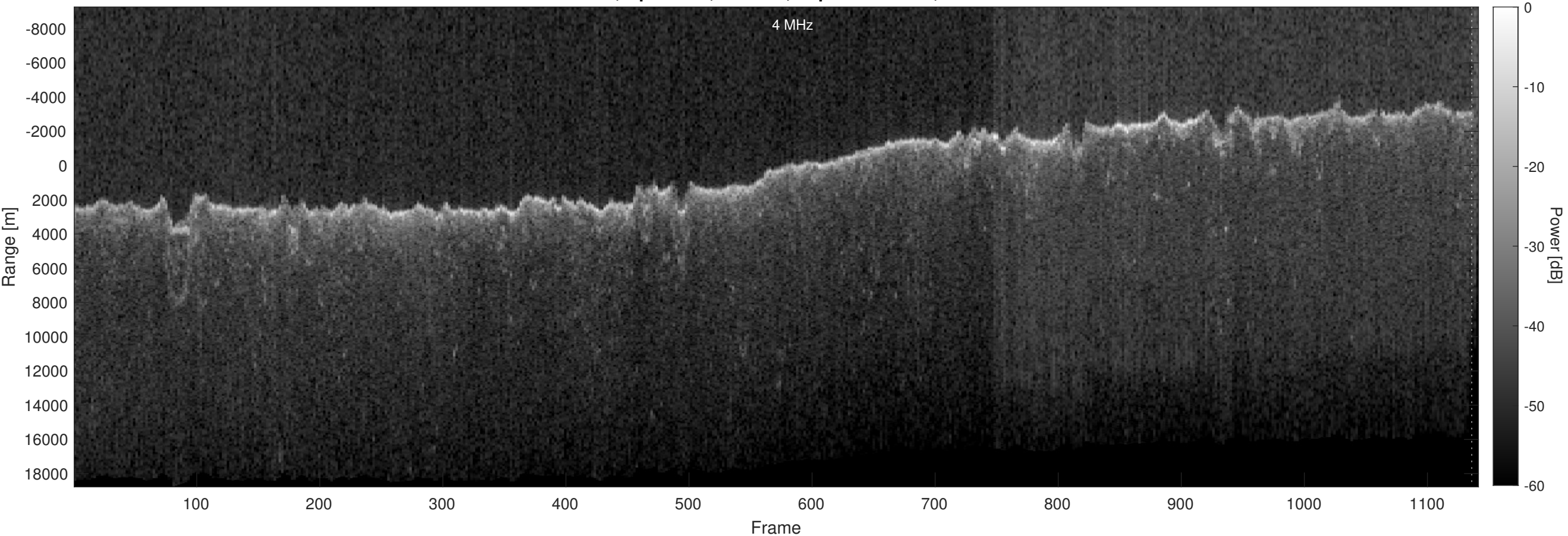
Orbit 11234, Optimized, Window, Depth-Corrected, Channel 2
