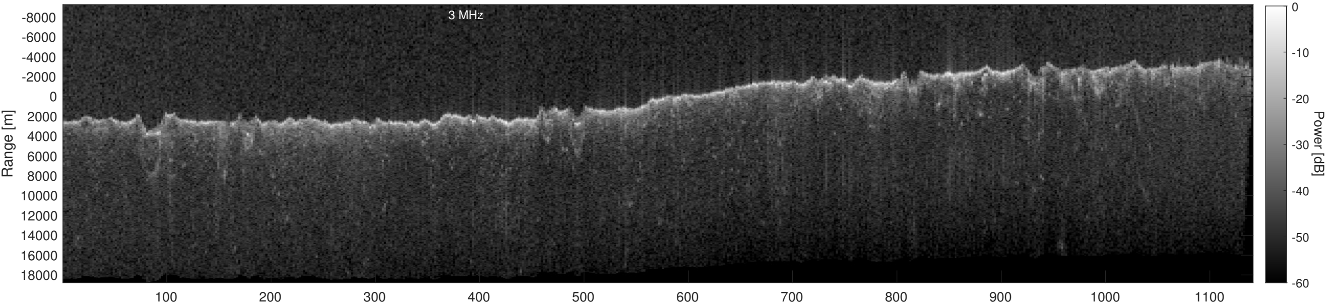
Orbit 11234, Depth-Corrected Cluttergram
