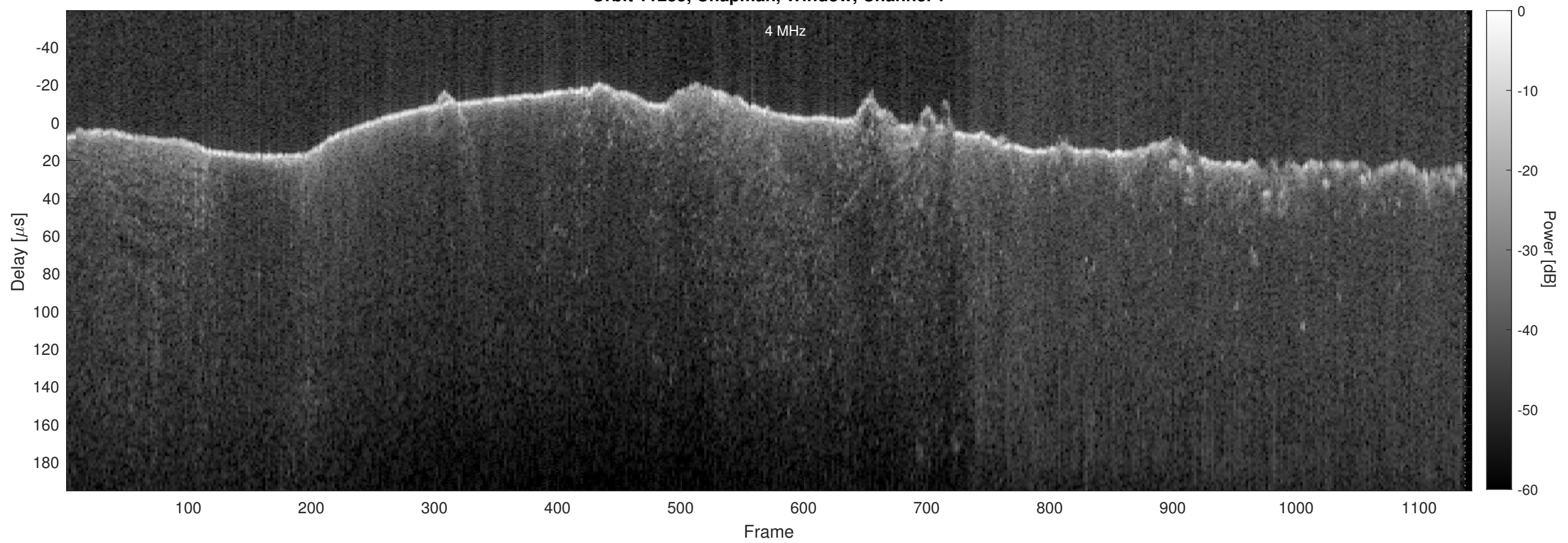
Orbit 11235, Chapman, Window, Channel 2
