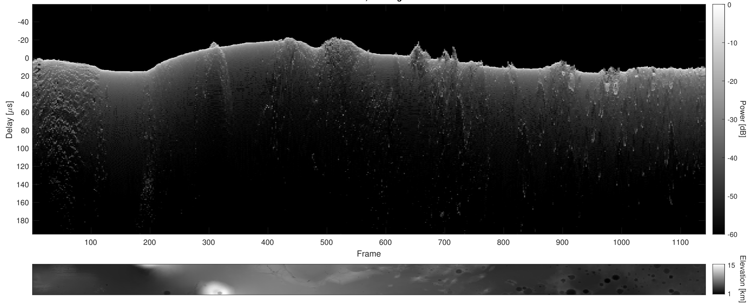
Orbit 11235, Cluttergram
