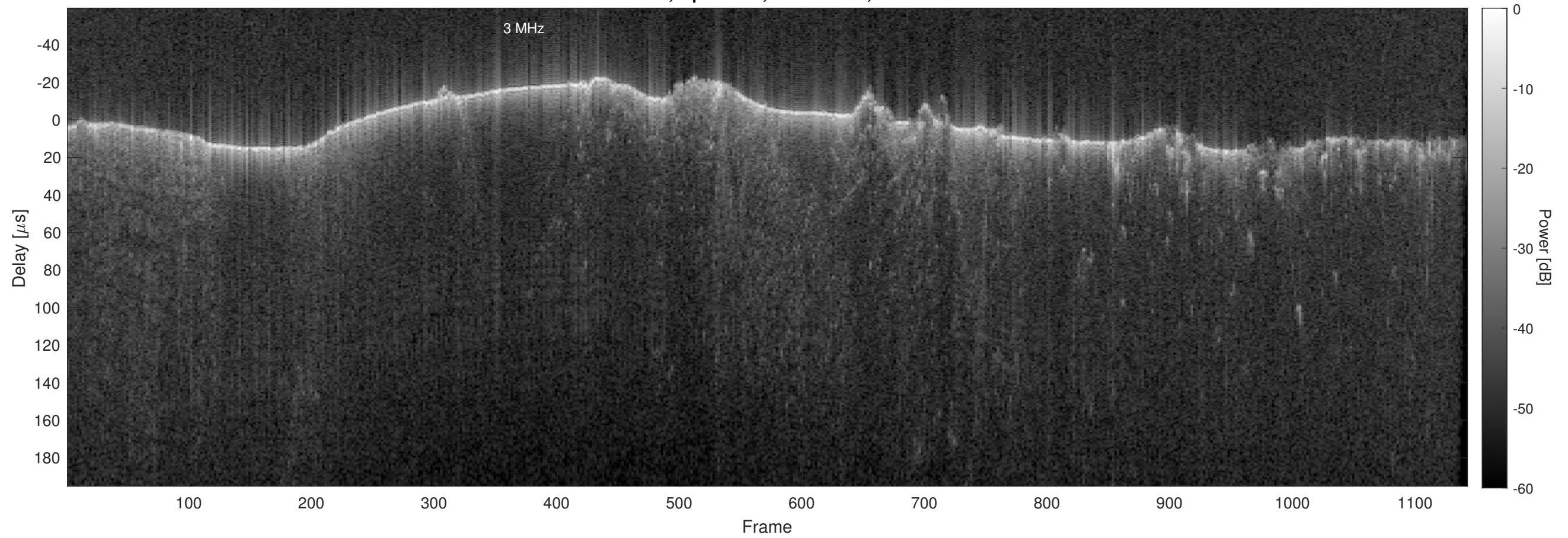
Orbit 11235, Optimized, No Window, Channel 2
