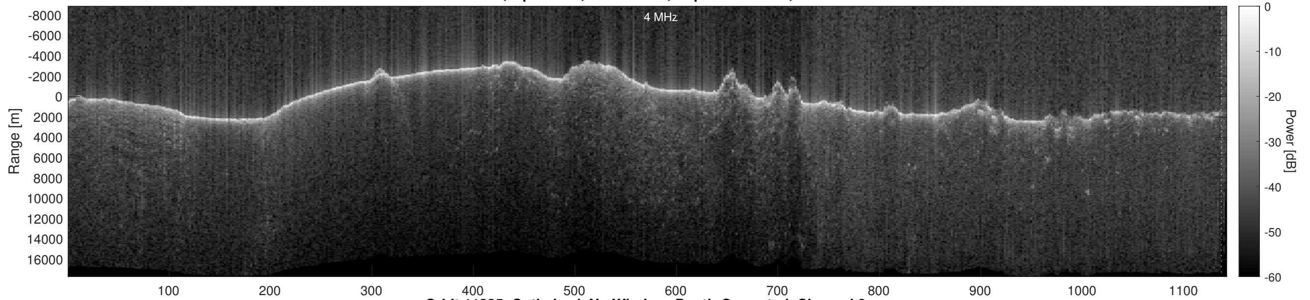
Orbit 11235, Optimized, No Window, Depth-Corrected, Channel 2
