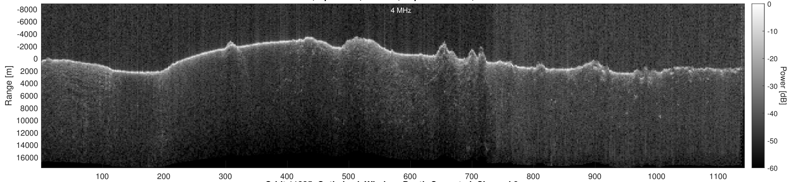
Orbit 11235, Optimized, Window, Depth-Corrected, Channel 2
