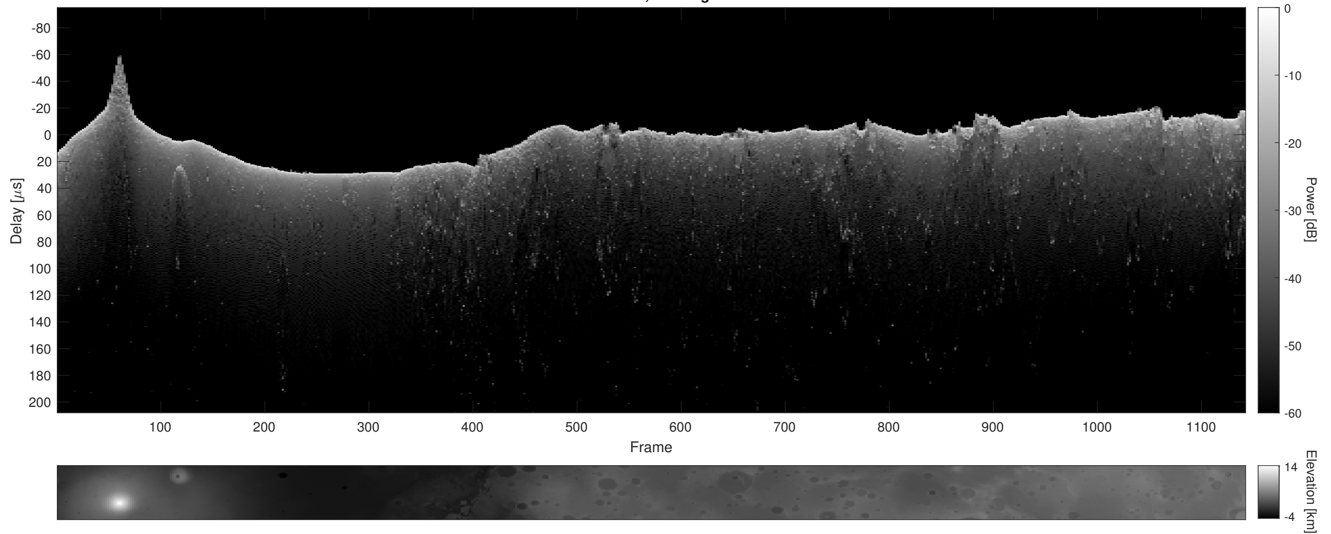
Orbit 11236, Cluttergram
