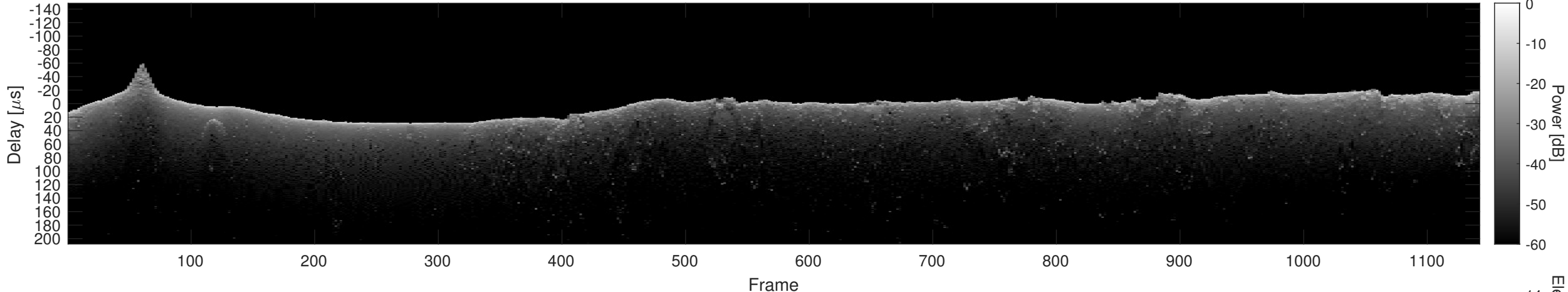
Orbit 11236, Cluttergram
