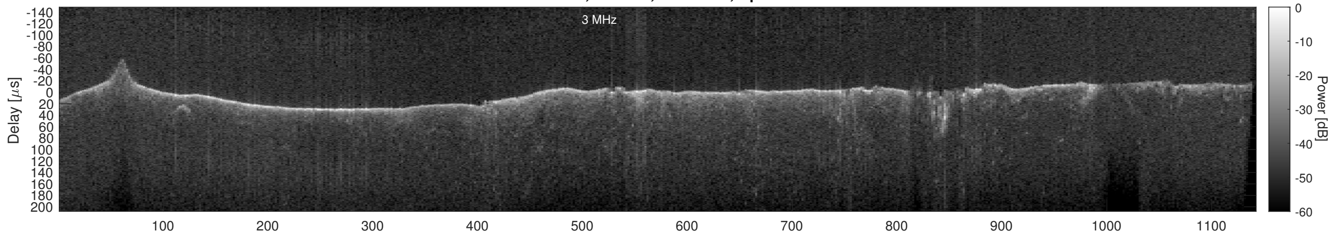
Orbit 11236, Cluttergram
