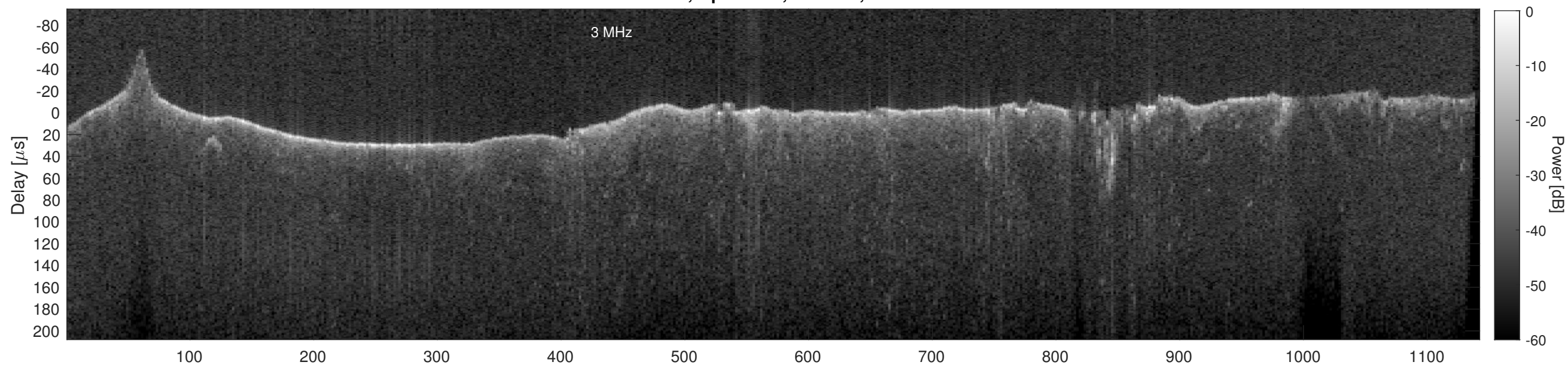
Orbit 11236, Cluttergram
