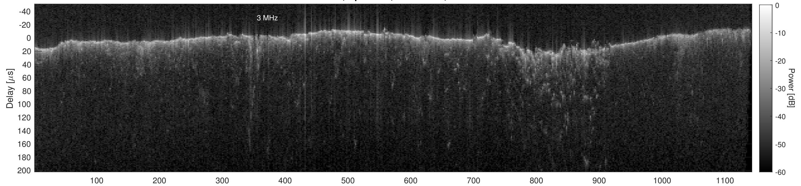
Orbit 11237, Cluttergram
