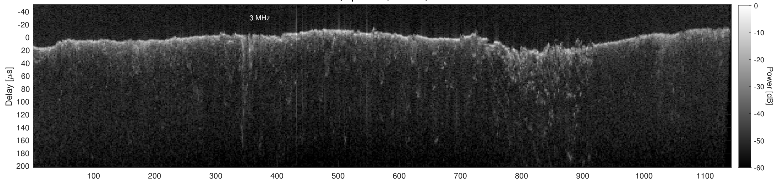
Orbit 11237, Cluttergram
