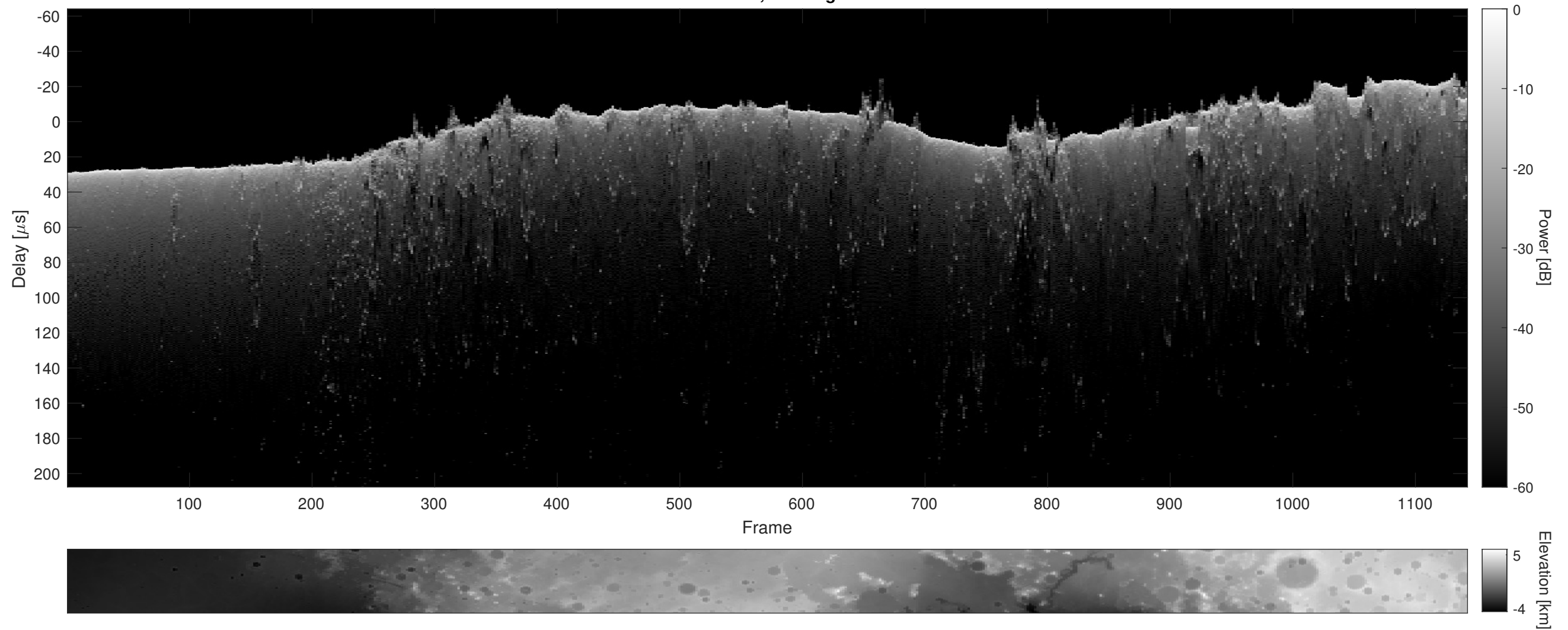
Orbit 11240, Cluttergram
