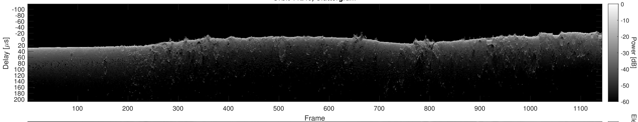
Orbit 11240, Cluttergram
