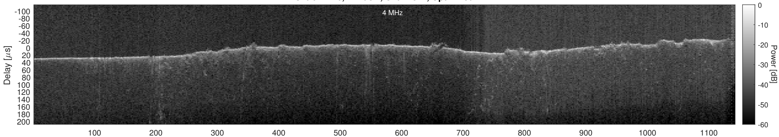
Orbit 11240, Cluttergram
